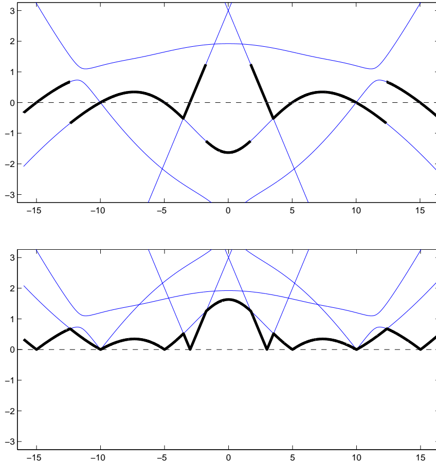
Figure 1: Eigenvalue and singular value curves for Example 5.5
