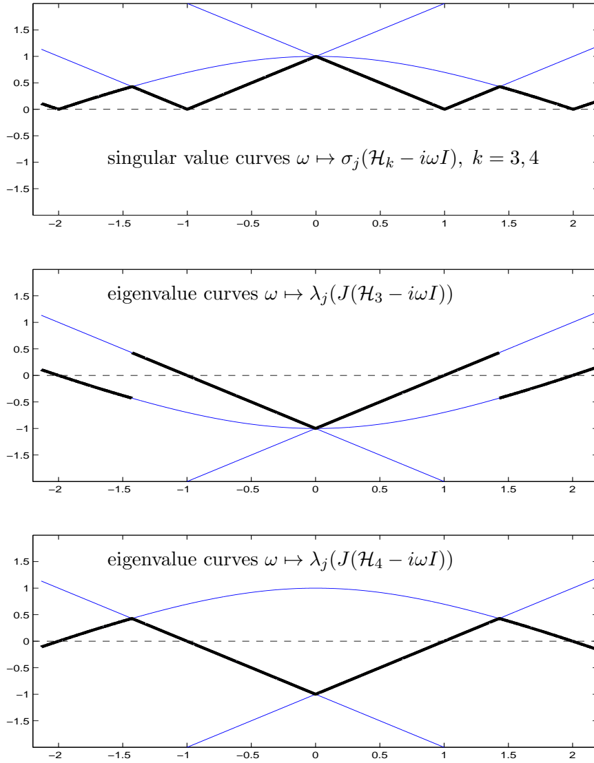
Figure 2: Eigenvalue and singular value curves for Example 5.14.
