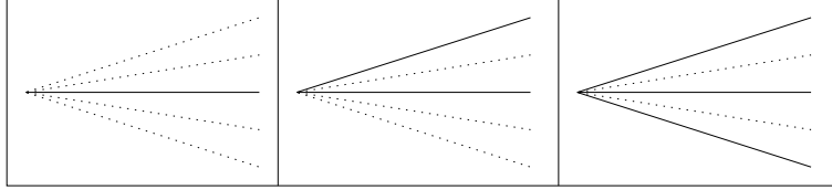
Figure 1: Illustration of selecting the first, second and third scenario out of N = 5
