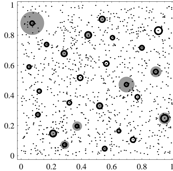
Fig. 5. N = 1000 samples \xi^i from the uniform distribution on [0,1]^2 and n = 25 points \xi^{u_k} , k = 1, \dots, n , obtained via the first 25 elements z_k , k = 1, \dots, n , of the Halton sequence (in the bases 2 and 3) (see [17, p. 29]). The probabilities q_k of \xi^{u_k} , k = 1, \dots, n , are computed for the distance d_\lambda with \lambda = 1 (gray balls) and \lambda = 0.9 (black circles) by solving (29). The diameters of the circles are proportional to the probabilities q_k , k = 1, \dots, 25 .
