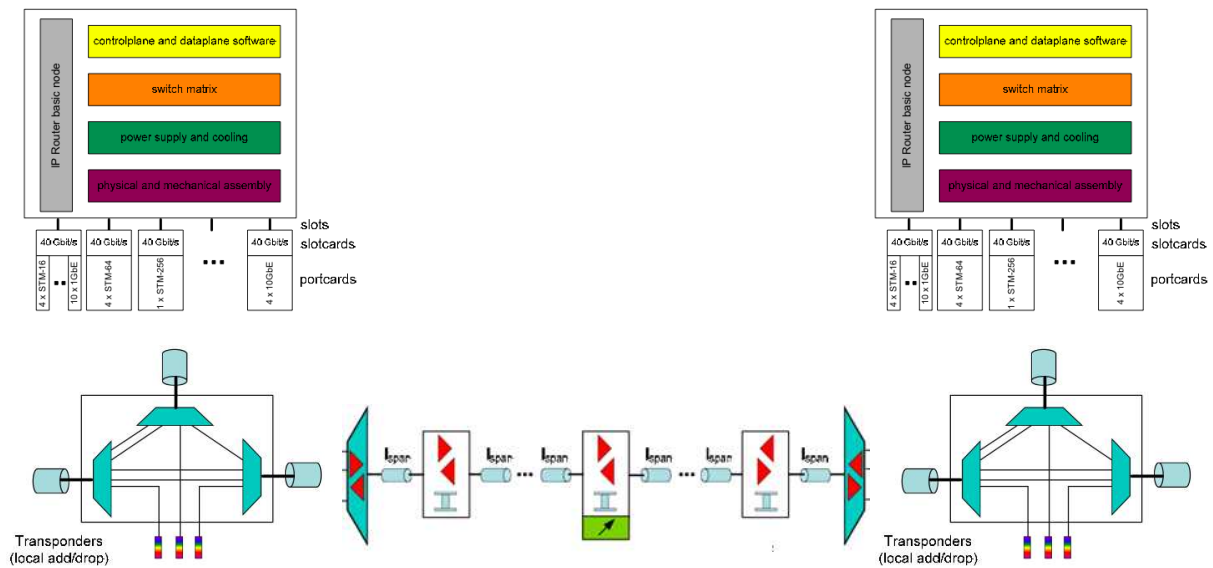
Figure 2: IP layer over WDM layer (Source: NOBEL hardware and cost model [6])
