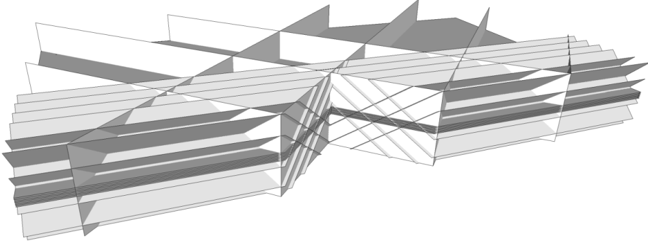
FIGURE 7. The affine arrangement \mathcal{A}_4 consists of three families of planes: The first family \mathcal{A}'_3 \times \mathbb{R} forms a coarse vertical grid; the second family (derived from \mathcal{H}_3 \times \mathbb{R} by tilting) forms a finer grid running from left to right; the last family \mathcal{H}_4 contains the parallel horizontal planes.
