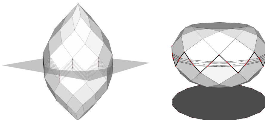
FIGURE 1. Eppstein’s Ukrainian easter egg, and its dual. The 2D-cut, resp. shadow boundary, of size \Omega(n^2) are marked.
