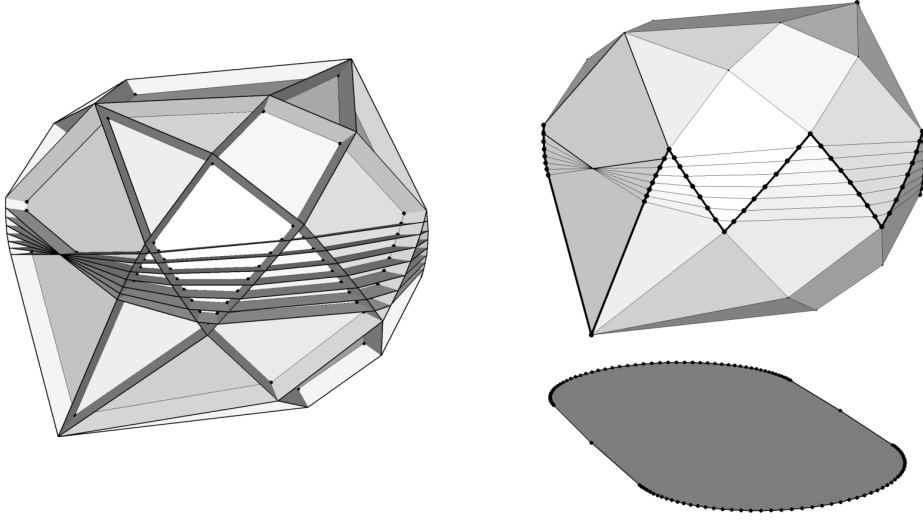
FIGURE 5. A dual 3-zonotope with quadratic 2D-shadow, on the left with the corresponding linear arrangement and on the right with its 2D-shadow.
