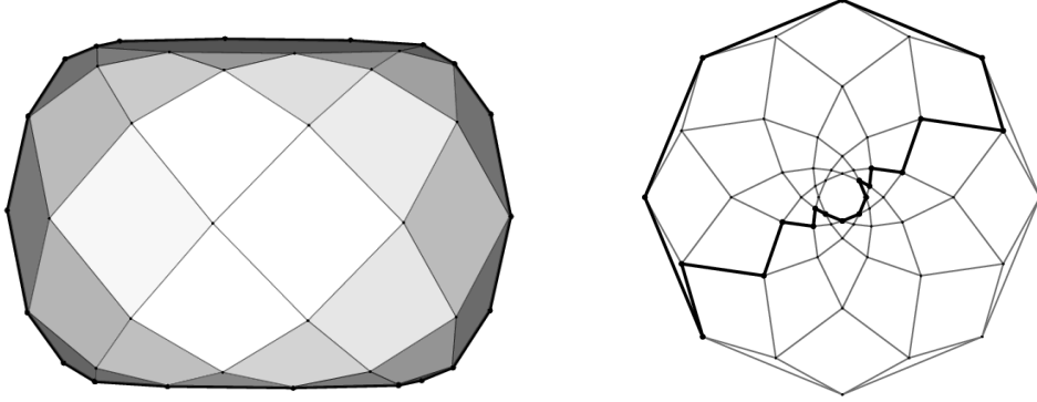
FIGURE 4. Shadow boundary of a centrally symmetric 3-polytope, on the right displayed as its Schlegel diagram.
