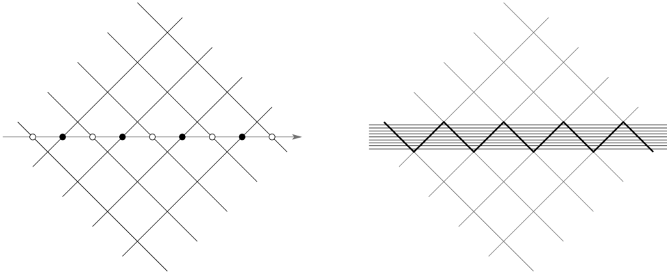
FIGURE 6. Constructing the arrangement \mathcal{A}'_3 from \mathcal{A}_2 (left) and \mathcal{A}_3 from \mathcal{A}'_3 (right).
