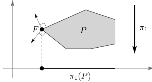
FIGURE 3. Survival of a face F in the projection \pi_1 to the first coordinate.
