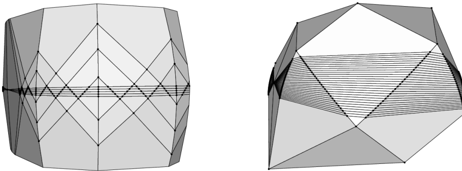
FIGURE 8. Two different projections of a dual 4-zonotope with cubic 2D-shadow. On the left the projection to the first two and last coordinate (clipped in vertical direction) and on the right the projection to the first three coordinates.
