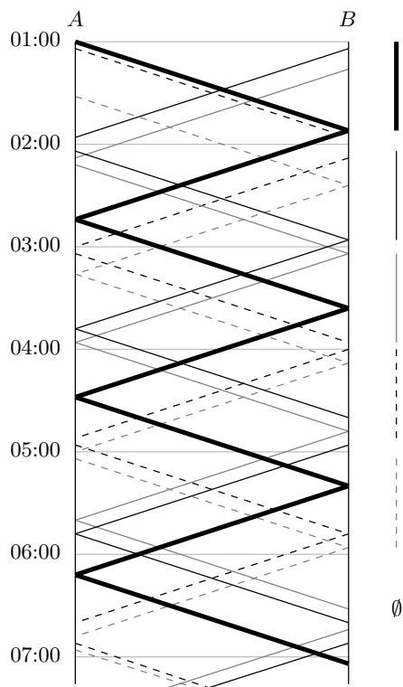
Fig. 2. A timetable for t_{ab} = t_{ba} = 52 , that uses only five vehicles. In the first five hours, there are three departures from each terminus station. But in the sixth hour, there are only two departures from B , which makes this timetable infeasible for N = 6 . The lines on the right indicate the vehicle that covers two trips in the corresponding hour.
