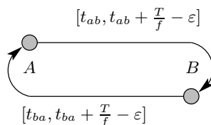
Fig. 1. The so-called PESP-graph (see, e.g., [2]) for the situation of the periodic vehicle circulation as it is considered in Prop. 1.
