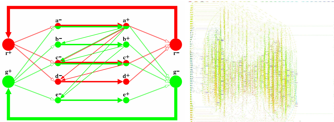
Figure 1: A vehicle scheduling graph for a 2-depot problem (left) and a duty scheduling graph (right); note the morning and the afternoon peaks on the right.
