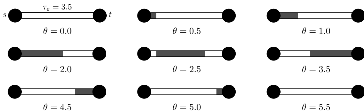
Figure 1: Snapshots of the simple flow over time discussed in Example 2.2 for several points in time. At time 0, the arc e = (s, t) (directed from left to right) is empty and we start to pump flow at rate 1 into the arc. At time 0.5 we have pumped half a unit of flow into the arc, at time 2 there are two flow units and we stop pumping. The first flow particles of the first flow unit reach the head node t at time \tau_e = 3.5 . At time 4.5 the first flow unit has arrived at node t while the second flow unit is still on the arc. Finally, at time 5.5 the last flow particles have arrived at node t and the arc is empty again.
