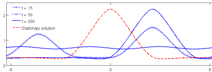
Figure 4: Evolution of a solid film governed by (51) from a nearly-uniform initial profile and anisotropy strength G = 0.1 . At long times, triangular shaped islands form, collapse, and the shifted profile approaches that given by the steady state solution described in Section 4.2 (dashed curve).
