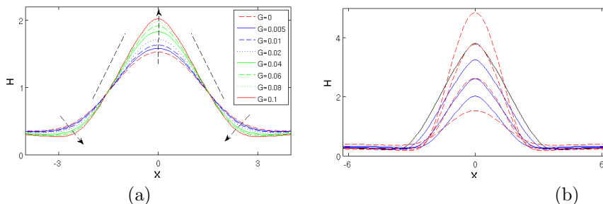
Figure 5: Steady profiles for periodic solutions. (a) Increasing surface energy anisotropy strength G , with fixed film volume V . (b) Increasing V from V = 2.6\pi to V = 4.8\pi ; for G = 0.1 , leads to a family of faceted islands (solid lines). With constant surface energy, width remains approximately constant (dashed lines).
