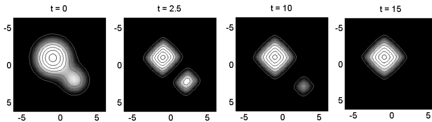
Figure 8: Collapse of a Ge/Si dot. Bright colors show bigger values of the surface height. The initial condition for these two islands were two round, exponential humps that initially evolve to faceted structures. The bigger quantum dot "eats" the smaller one and survives. The simulation has been carried out with G = 0.2 . Time and space are given here and in the other figures in dimensionless units.
