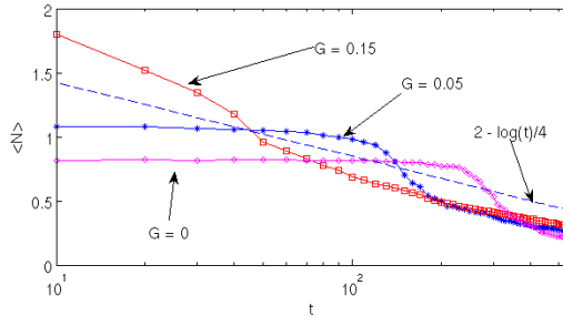
Figure 7: Coarsening diagram for the 2D Ge/Si system comparing dot densities for the isotropic ( G = 0 ) and two anisotropic trials ( G = 0.05 and G = 0.15 ). One trial is the average of four runs and the t -axis is logarithmic.
