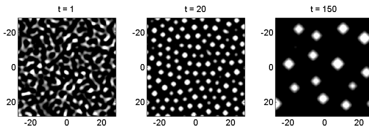
Figure 9: Simulation of the Ge/Si system. An initially randomly perturbed surface first evolves into round dots that coarsen in time and during their growth change their shape to small pyramids.
