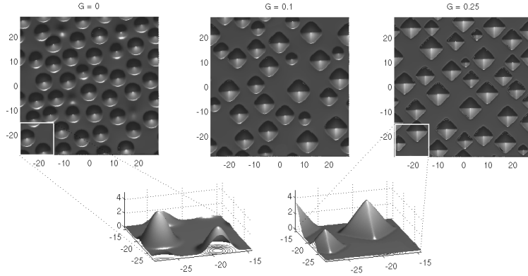
Figure 10: Anisotropy effect on the 3D Ge/Si system. All three pictures show the same time-point after evolution from the same initial condition (random perturbation of a flat state). The upper left shows a simulation with isotropic surface tension ( G = 0 ) and the dots have round tips. In the other two pictures ( G = 0.1 and G = 0.25 ) we observe faceting which is stronger for the bigger anisotropy coefficient G .
