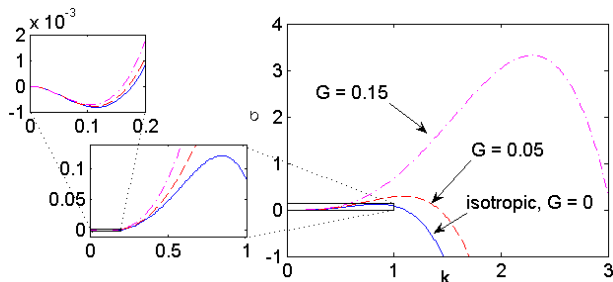
Figure 2: Dispersion relation for the isotropic ( G = 0 ) and the anisotropic cases G = 0.05 and G = 0.15 with \bar{H} = 0.8 . On the left we see a magnifications of the wave number regime where the minimum is adopted.
