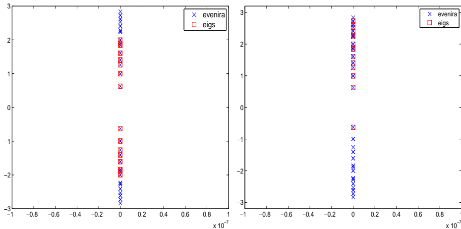
FIG. 7.1. Example 7.1. Eigenvalues of (M, N) closest to \sigma = 1 (left) and to \sigma = i (right) approximated with eigs and with Even-IRA
