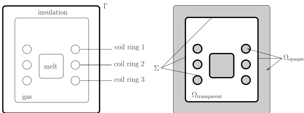
Figure 1: Two-dimensional schematic cut of the domain \Omega . Left-hand: The furnace components and the outer boundary \Gamma (thick black line). Right-hand: Description of \Omega from the point of view of heat radiation, with the transparent cavity \Omega_{\text{transparent}} (white), its boundary \Sigma , (thick black line) and the opaque materials \Omega_{\text{opaque}} (grey).
