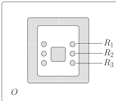
Figure 2: Two-dimension cut of the Maxwell 'hold all domain' O , with the electrical conductors O_c (gray), the nonconductors O_{nc} (white), and the coil rings R_1, \dots, R_3 indicated by arrows.
