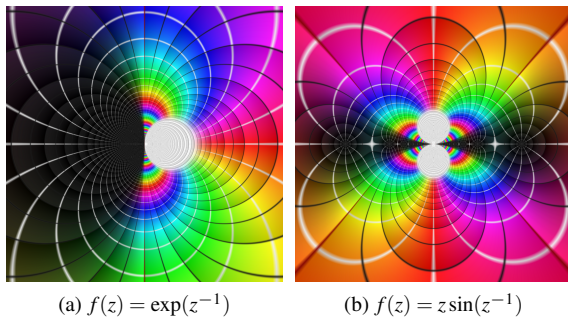
Figure 5: Essential singularities
