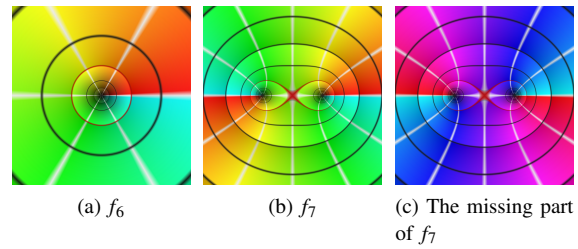
Figure 10: Discontinuity arising from square roots
