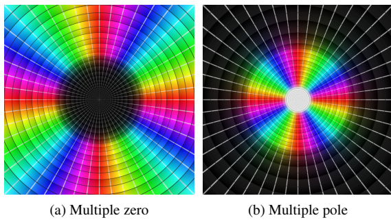
Figure 4: Typical pattern of a multiple zero z^k and a multiple pole z^{-k}
