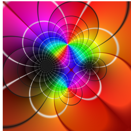
Figure 3: Plot of the rational function f_1
