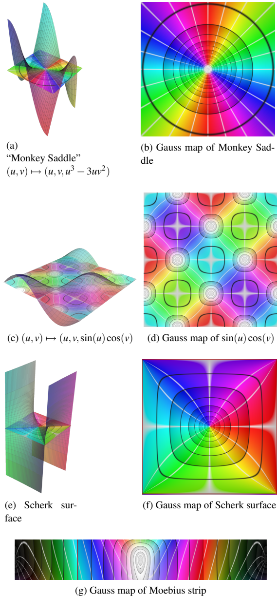
Figure 12: Domain colored Gauss maps
