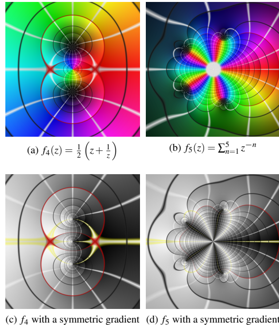
Figure 8: Visualizing the Schwarz reflection principle
