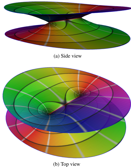
Figure 11: Riemann surface for f_7
