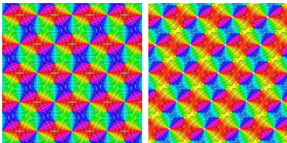
(a) \wp -function, \tau = 0.5 + 0.5i (b) \wp -function, \tau = 0.2 + 0.8i
