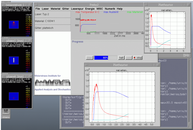
Figure 5: Screenshot of WIAS-SHaRP.
