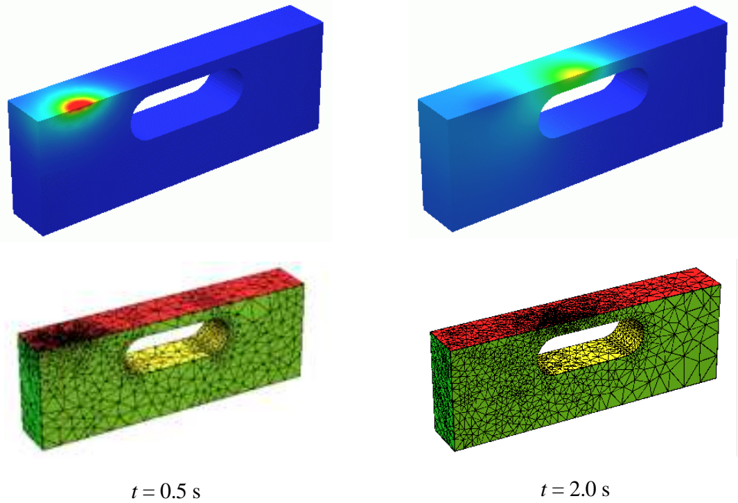
Figure 4: Temperature distribution and adaptive grid at two different times.
