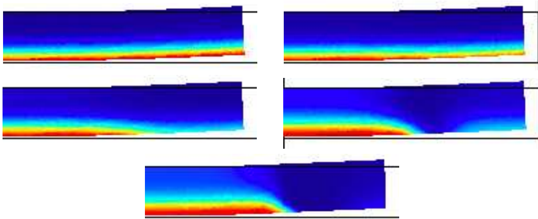
Figure 10: Five iterations of the gradient method.
