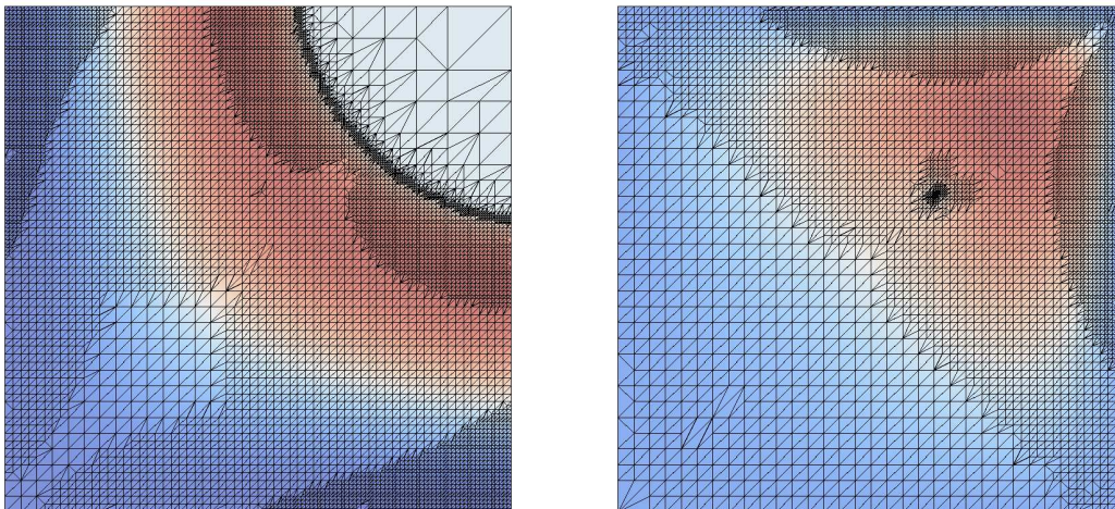
Figure 6: Computational grids for both problems, near \mu = 10^{-6} .
