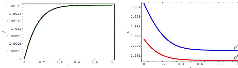
Figure 3: Radius of the grain r_0 and mass densities in ferrite \rho^\alpha and austenite \rho^\gamma .
