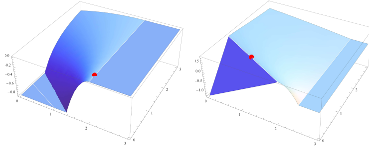
Figure 2: Plot of profit functions for a solution of the two generators EPEC
