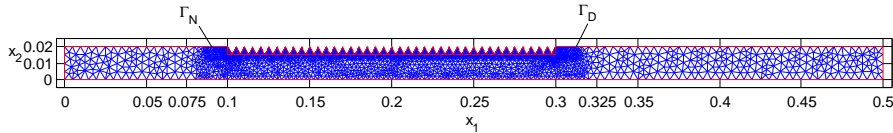
Fig. 7.1: Computational domain.
