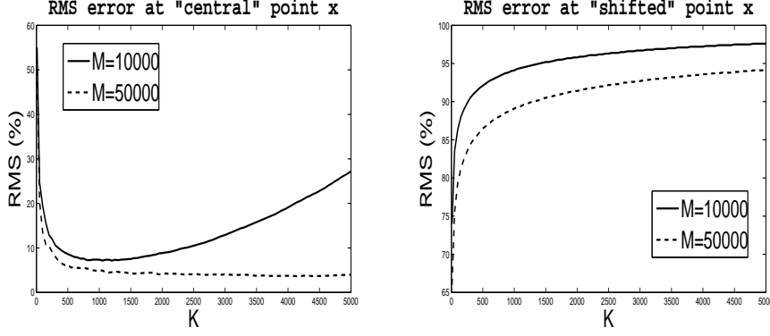
Figure 1: Root-mean-square errors (in %) of the estimators \widehat{C}_{2,10000}^{knn}(x, 0) (solid line) and \widehat{C}_{2,50000}^{knn}(x, 0) (dashed line) for different numbers k of nearest neighbors at two points x_0 \exp(-\sigma^2) (left) and x_0 \exp(-\sigma^2 + 1.5(\sigma\sqrt{\delta_0} + \sigma\sqrt{\delta_1})) (right).
