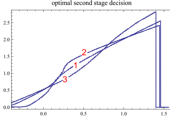
Figure 3: Second stage release policies for the previous example (at l_0 = 1.7 ) but with an assumed correlation between inflow components of \rho = -0.3 (1), \rho = 0 (2) and \rho = 0.9 (3), respectively.
