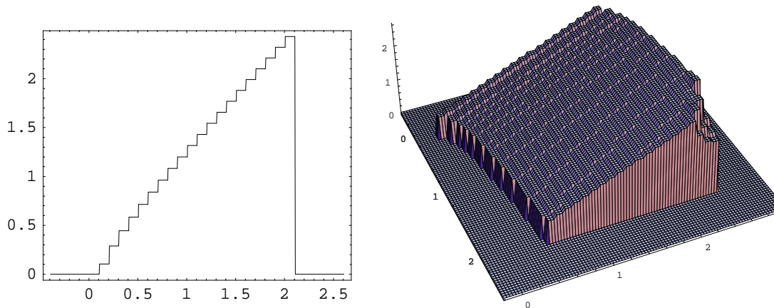
Figure 5: Optimal second stage and third stage release policies for a three-stage example with independent components
