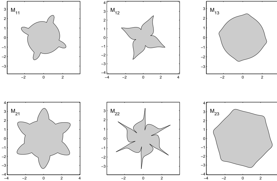
FIG. 5.1. The limit sets \mathcal{L}_\lambda of the matrices in Example 5.1 .
