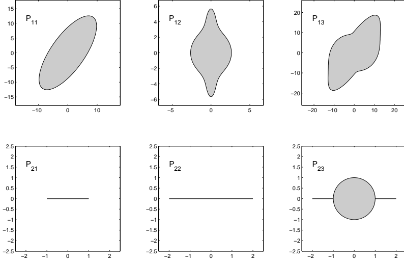
FIG. 5.2. Limit sets of the projectors in Example 5.2
