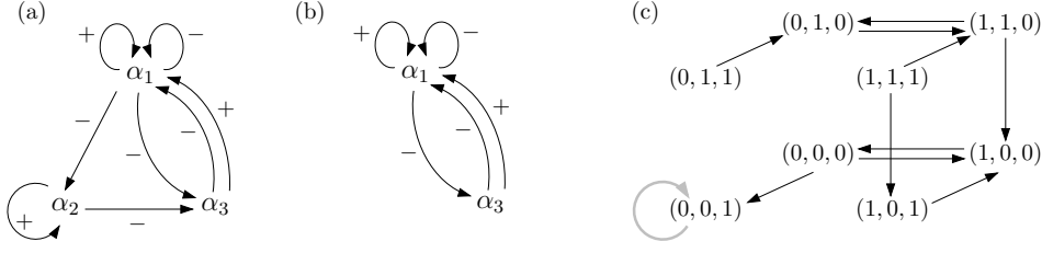
FIGURE 5. We choose the parameters for the interaction graph in (a) as K_{1,\{e_{11}^+,e_{31}^+\}} = K_{1,\{e_{11}^-,e_{31}^-\}} = K_{2,\{e_{12}^-,e_{22}^+\}} = K_{3,\{e_{13}^-,e_{23}^-\}} = 1 and set all other parameters 0. In (b) the graph \mathcal{I}^\theta(s) for the singular steady state s = (\theta, 0, \theta) . In (c) the corresponding state transition graph.
