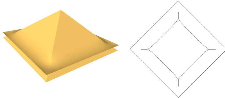
FIGURE 3. Approximate solution u_{12} with obstacle function \psi and associated free boundary
