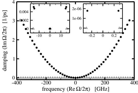
Figure 6: Main roots \Omega of Eq. (9) (black bullets) and their initial approximations given by Eq. (10) (grey triangles) for some fixed \beta(z) with \langle\bar{\beta}\rangle = 0 . Inserts: the vicinity of the zero frequency showing closely located pairs (\Omega_{k+}, \Omega_{k-}) . Parameters \kappa , \Delta , \Delta_\alpha , \varepsilon_{Is} , \varepsilon_{Ic} , \bar{\omega} are set to zero. \varepsilon_{Gs} = \varepsilon_{Gc} \neq 0 , R = 0.1 , T = \sqrt{0.7} .
