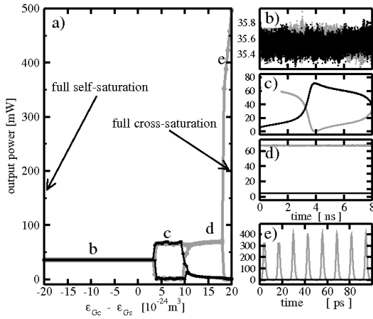
Figure 5: Dynamic regimes for different contributions of the cross- and self-gain saturations. (a): maximal and minimal intensities of the emitted field for different values of \epsilon_{Gc} - \epsilon_{Gs} . (b-e) typical representatives of the observed regimes. Grey and black: CW and CCW propagating fields. A small distributed coupling ( \kappa|S| = (10 + 0.4i) \cdot 10^{-3} , |S| : length of the ring cavity) was assumed. \epsilon_{Gs} + \epsilon_{Gc} = 20 \cdot 10^{-24} \text{ m}^3 .
