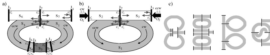
Figure 1: Schemes of several ring laser configurations with indication of sections ( S_r ), junctions ( J_r , black intervals), optical injections ( O_r , thick black arrows), propagation directions of the CW and CCW fields (thin black arrows) and some field transmission - reflection - outcoupling directions (grey arrows). (a): an all-active modelocked ring laser with a saturable absorber and (b): a simple ring laser with optical injections as considered in this paper. (c): some other ring laser devices [1, 2, 3, 16] which can be also treated by our software.
