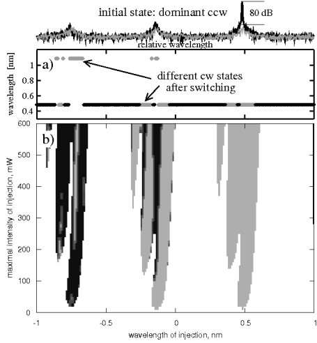
Figure 4: Switching of the initial CCW field (top) by injecting a CW propagating and 100 ps long optical pulse in dependence on the wavelength and the maximal intensity of this pulse. (a): wavelength of the dominant field after the propagation of the injected pulse with 200 mW maximal intensity. Here and at the top: grey and black correspond to the CW and CCW fields. (b): different grey shadings represent the wavelength of the CW field after the successful switching.
