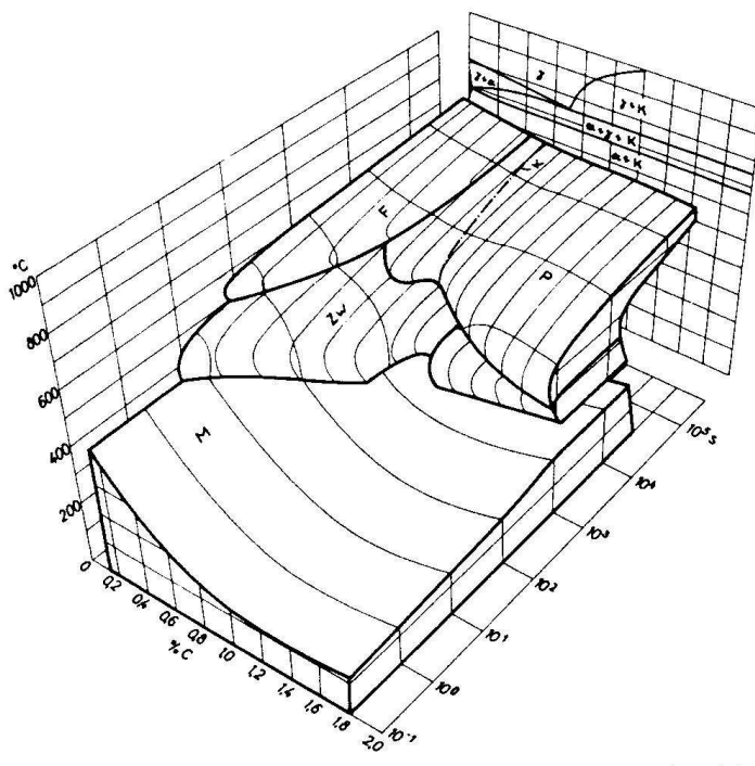
Figure 2: Three-dimensional presentation of the transformation characteristic of a 14NiCr14 steel, for continuous cooling, after austenization at 1023^{\circ}K (Symbols: ZW bainite, M martensite, P pearlite, F ferrite).
