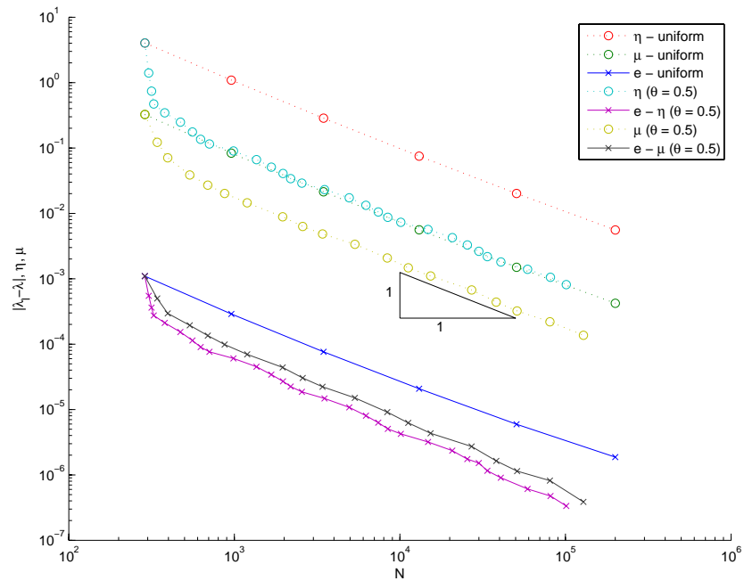
FIGURE 6.15. Convergence history for the first eigenvalue \lambda_1 = 0.001191353227676 of the tuning fork.
