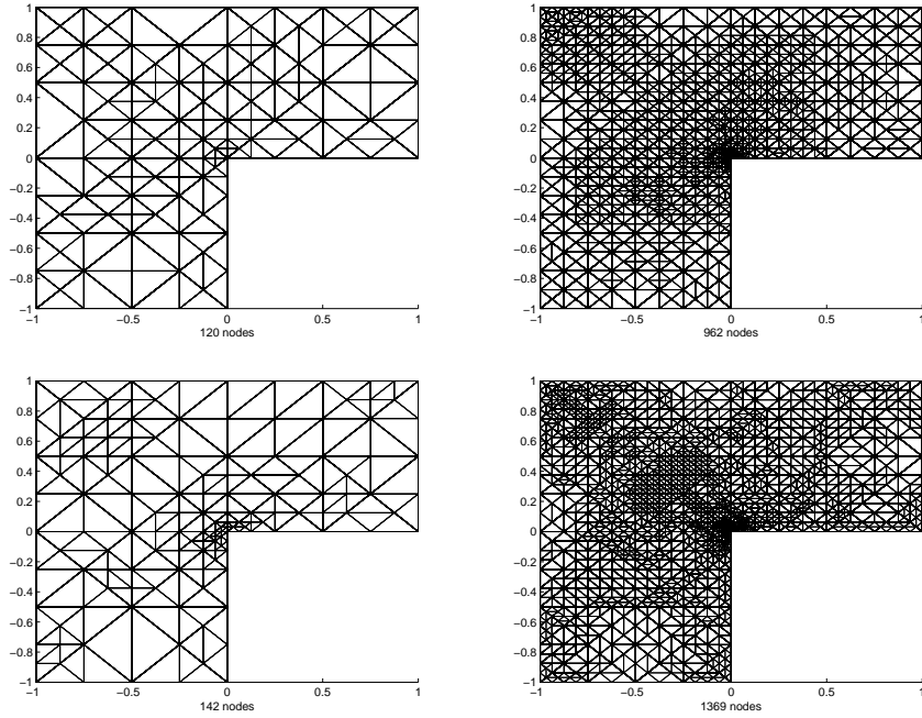
FIGURE 6.6. Adaptive meshes generated with \theta = 0.5 for the a posteriori error estimator \eta_\ell (top) and \mu_\ell (bottom) for about 100 and 1000 nodes for the L-shaped domain.
