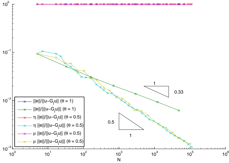
FIGURE 6.8. Size of the constant C with \|u - u_\ell\| \leq C\|u - G_\ell u\| and higher order convergence of the L^2 -norm compared to the energy norm for the L-shaped domain.
