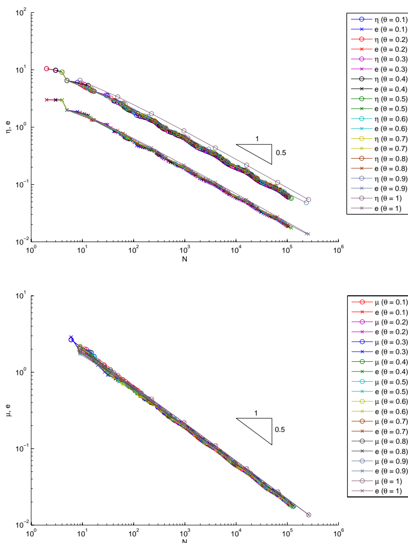
FIGURE 6.2. Convergence history for \eta_\ell (top) and \mu_\ell (bottom) with different choices of \theta for the unite square.
