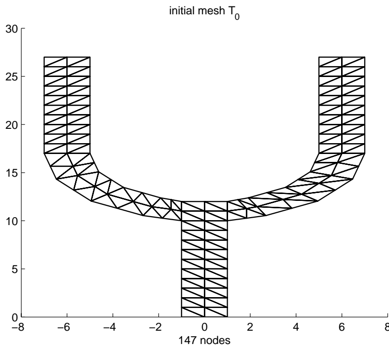
FIGURE 6.13. Initial triangulation T_0 for the tuning fork.
