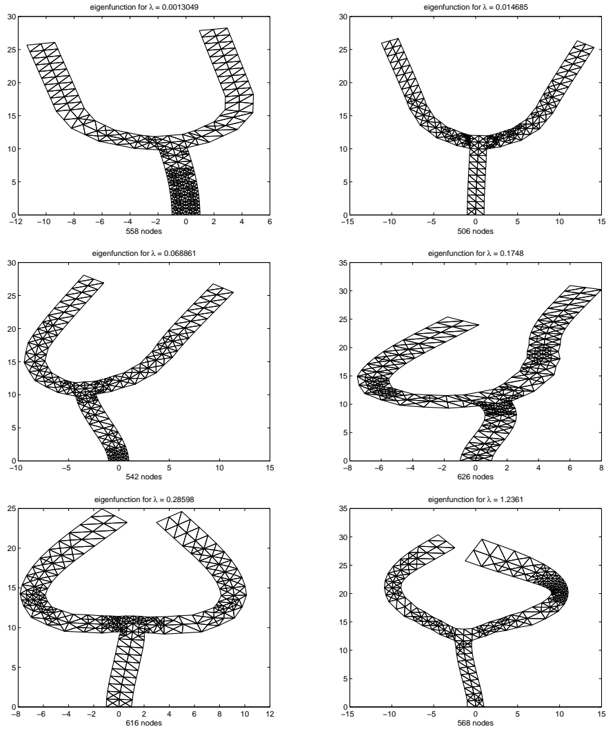
FIGURE 6.14. The first six eigenforms of the tuning fork computed on adaptively refined meshes for the corresponding discrete eigenvalue on level \ell = 7 with about 500 nodes, stretched by a factor 20.
