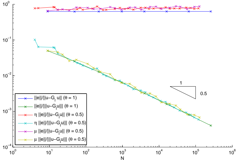
FIGURE 6.4. Size of the constant C with \|u - u_\ell\| \leq C \|u - G_\ell u\| and higher order convergence of the L^2 -norm compared to the energy norm for the unite square.
