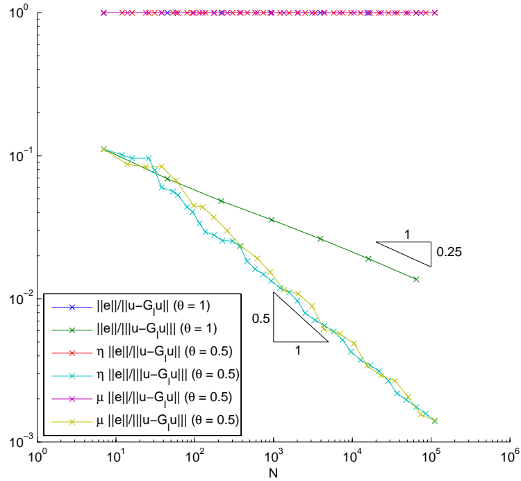
FIGURE 6.9. Size of the constant C with \|u - u_\ell\| \leq C\|u - G_\ell u\| and higher order convergence of the L^2 -norm compared to the energy norm for the slit domain.
