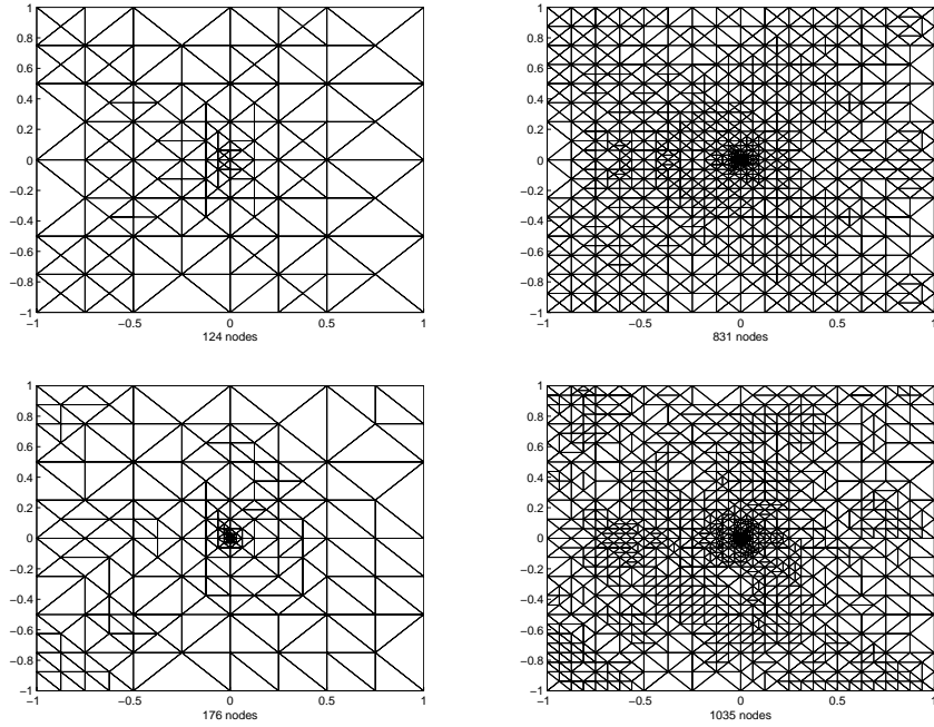
FIGURE 6.11. Adaptive meshes generated with \theta = 0.5 for the a posteriori error estimator \eta_\ell (top) and \mu_\ell (bottom) for about 100 and 1000 nodes for the slit domain.
