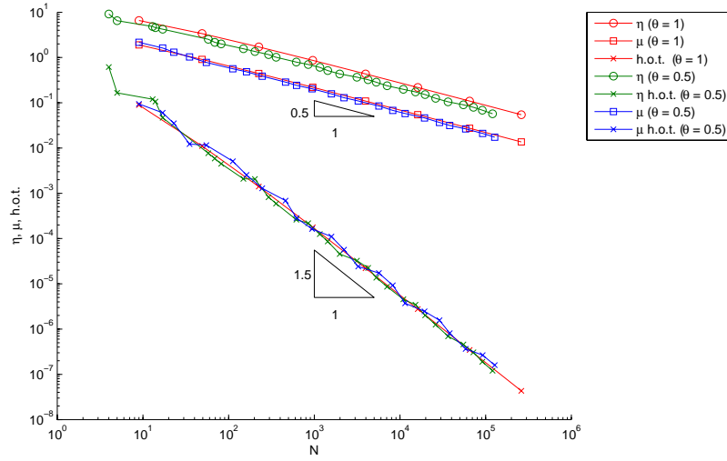
FIGURE 6.3. Comparison of the estimator and the h.o.t. for \eta_\ell and \mu_\ell for the unite square.
