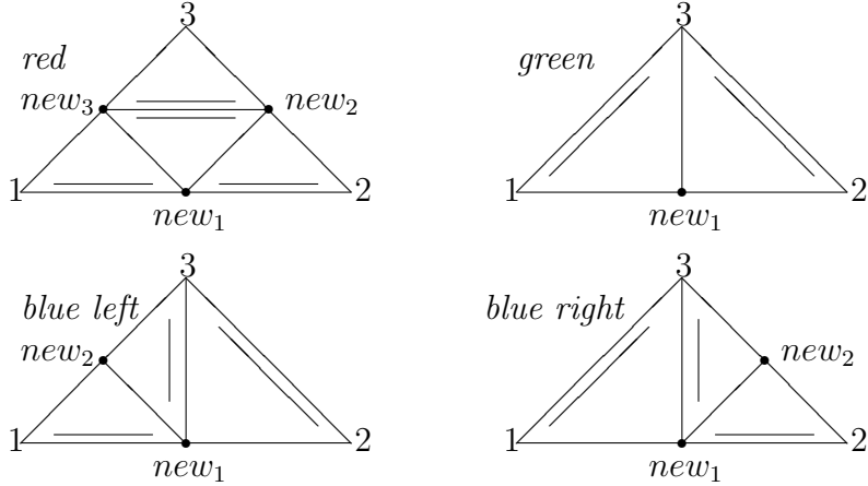
FIGURE 2.1. Red, green and blue refinement. The new reference edge is marked through a second line in parallel opposite the new vertices new_1 , new_2 or new_3 .
