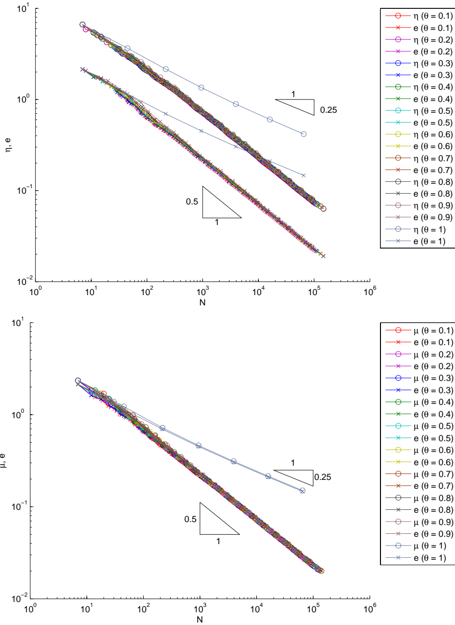
FIGURE 6.10. Convergence history for \eta_\ell (top) and \mu_\ell (bottom) with different choices of \theta for the slit domain.
