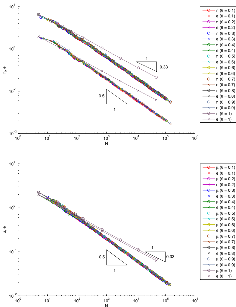
FIGURE 6.5. Convergence history for \eta_\ell (top) and \mu_\ell (bottom) with different choices of \theta for the L-shaped domain.
