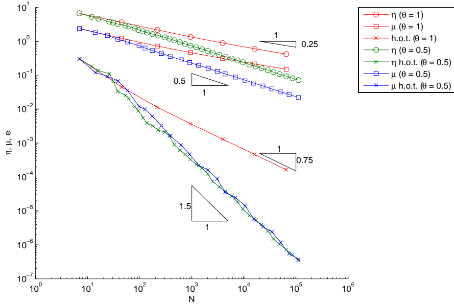
FIGURE 6.12. Comparison of the estimator and the h.o.t. for \eta_\ell and \mu_\ell for the slit domain.
