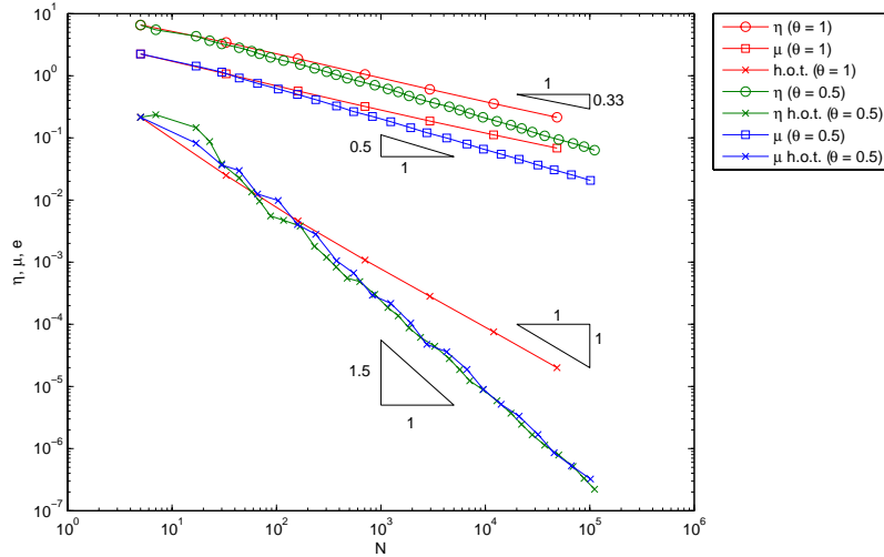
FIGURE 6.7. Comparison of the estimator and the h.o.t. for \eta_\ell and \mu_\ell for the L-shaped domain.
