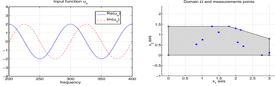
FIGURE 3. Run 2: Input function u_o for the frequencies from 200 to 400 Hz (left plot); observation points in \Omega \cup \Gamma_N (right plot).
