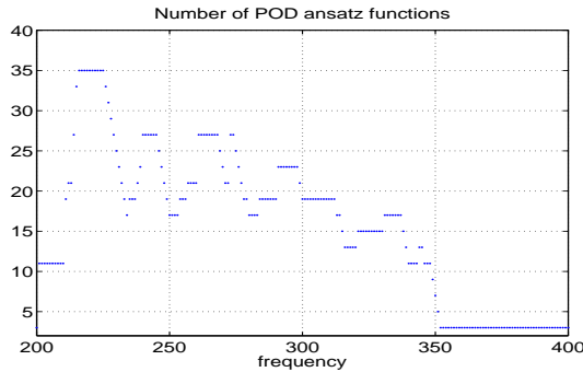
FIGURE 5: Change of the number \ell of POD basis functions.
