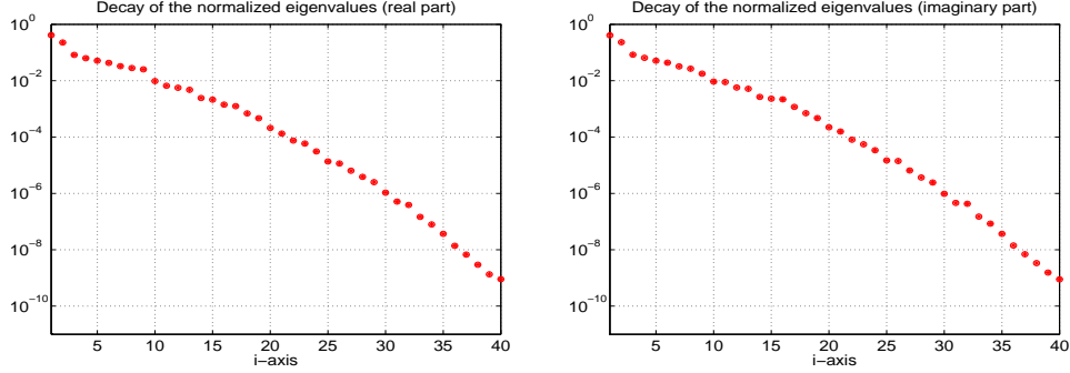
FIGURE 4. Run 2: Decay of the largest 40 normalized eigenvalues \lambda_i / \sum_{i=1}^d \lambda_i for the real and the imaginary part of the snapshots.
