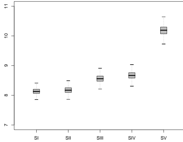
Figure 1: Upper bounds Y_0^{up}(\widehat{M}^\pi) , x_0 = 90 , D = 2 , with 95% confidence intervals for five different regression bases used for estimating \widehat{M}^\pi .
