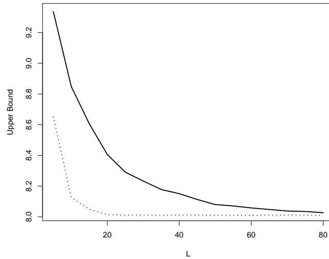
Figure 2: Upper bounds Y_0^{up}(0) (solid line) and Y_0^{up}(\widehat{M}^\pi) (dotted line) in dependence on the number of inner Monte Carlo paths L , the number of outer paths N being equal to 10000.
