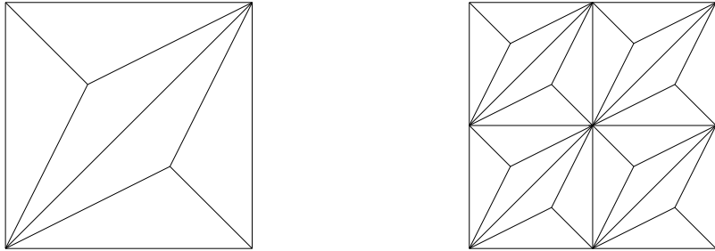
Figure 1: Two subsequent triangulations of the unit square with two and eight macro elements which result in six and 24 elements, respectively.
