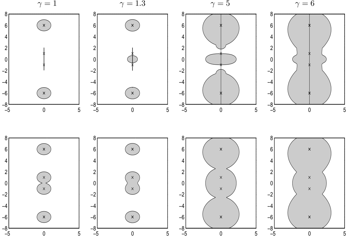
FIG. 7.1. The sets \sigma_{Ham}(H_\gamma; 1) (upper row) and \sigma_{\mathbb{C}^{n \times n}}(H_\gamma; 1) (lower row).
