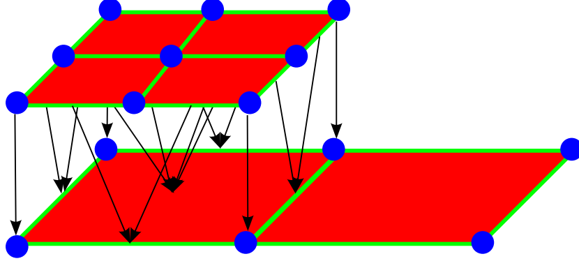
Figure 2: Father relation between two level grids.
