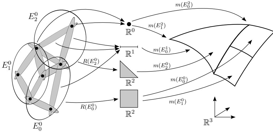
Figure 1: A 2-dimensional entity complex (left), the reference elements (center), and a geometric realization in \mathbb{R}^3 (right).
