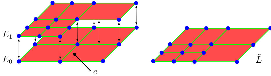
Figure 4: Copy relation between two entity complexes E_0 and E_1 (left), and corresponding leaf entity complex (right). Note that the edge e in E_0 is contained in \tilde{L} .
