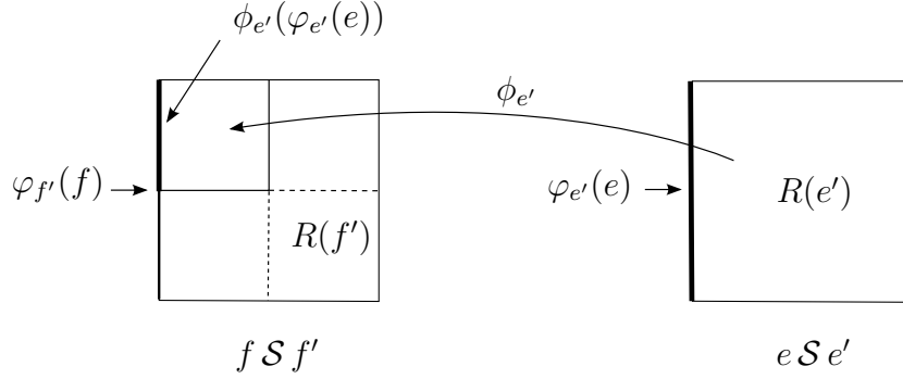
Figure 2: Father relation between two level grids.
