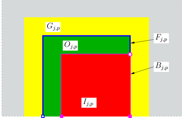
Figure 5: Data decomposition based on domain decomposition ideas.
