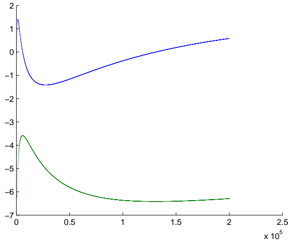
Figure 3: Graph of Steklov averages \psi_{H,i}(t) , i = 1, 2 , H = 500 .
