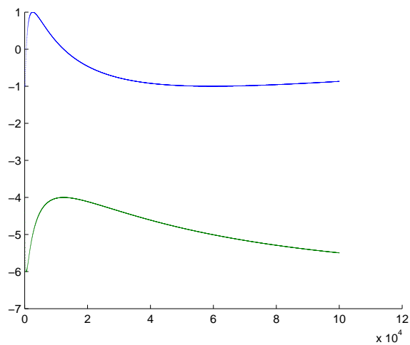
Figure 2: The graph of functions \lambda_i(t) , i = 1, 2 in Example 76.
