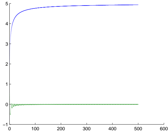
Figure 1: Graph of the functions \lambda_i(t), i = 1, 2 in Example 75.
