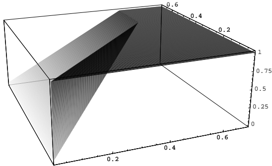
Figure 1: Cost function \xi \mapsto \Phi(\xi) from Example 1.1.
