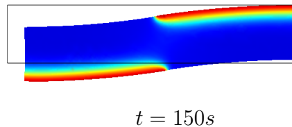
Figure 6: Distribution of phase martensite at time t = 150s . Blue corresponds to 0 % and red to 100 %, respectively.
