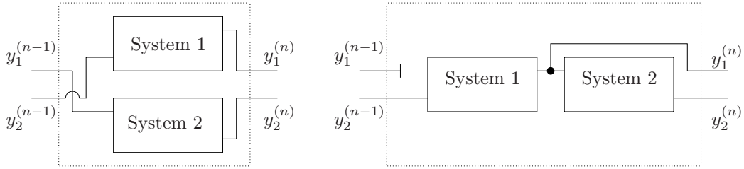
Figure 1: block diagram of the JACOBI method (left) and the GAUSS-SEIDEL method (right)
