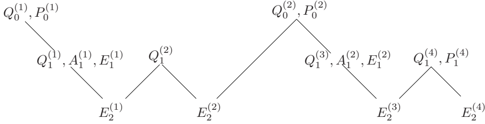
FIGURE 3.1. Illustration of the recursive construction of projectors in the index 2 case. Top down, we have the chain matrices in increasing order. From left to right, we have the successive calculation of these.
