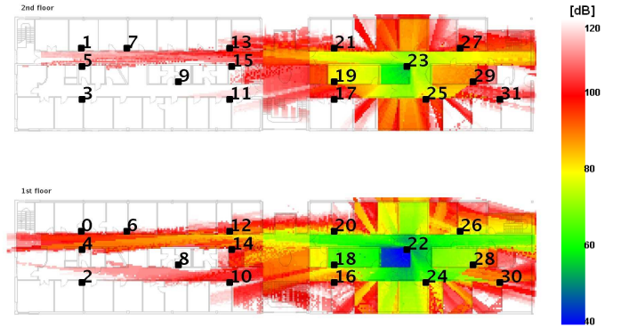
Fig. 3. Candidate APs locations and path-loss prediction for candidate AP 22
