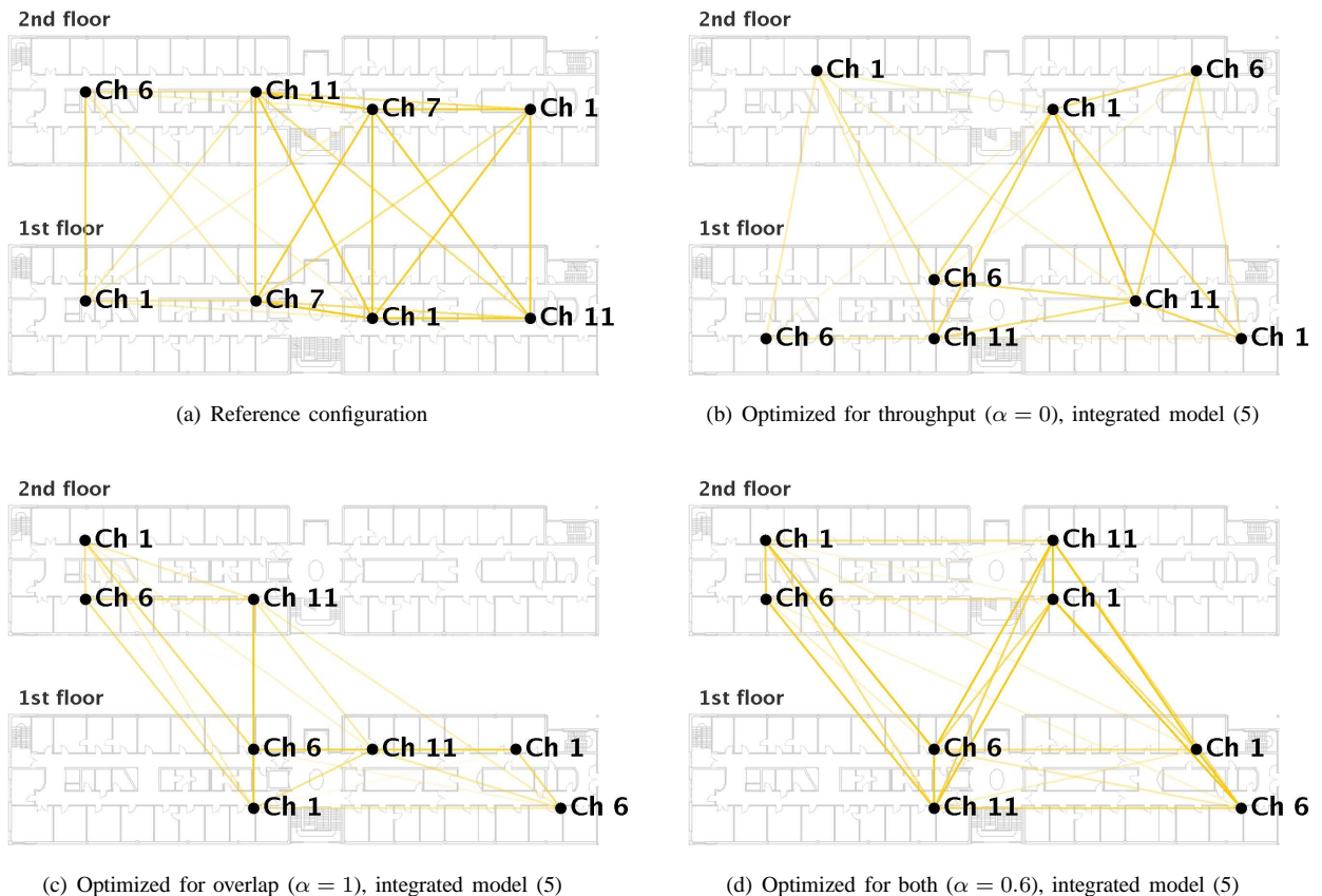
Fig. 5. AP positions and overlap for different network designs
