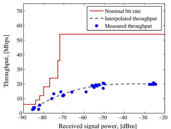
Fig. 1. Nominal and net throughput vs. received signal power
