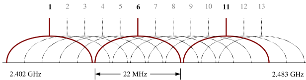
Fig. 2. Channels available for IEEE 802.11g
