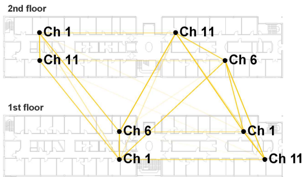
(a) Optimized solution by model (5), \alpha = 0.6 , 3 channels
