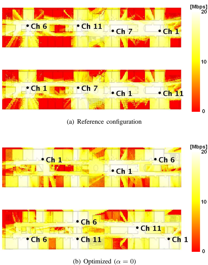
Fig. 4. Impact of optimization on throughput, integrated model (4)
