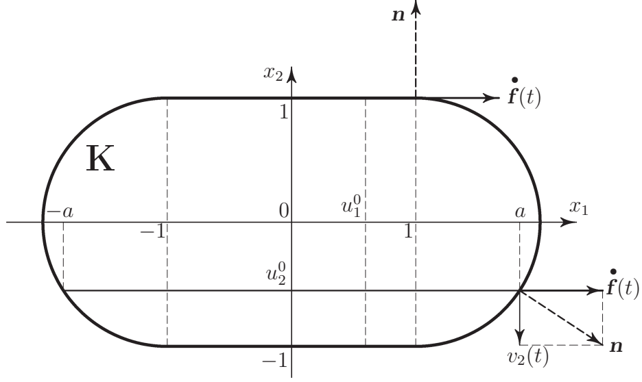
Figure 1: An illustration to Example 3.9.
