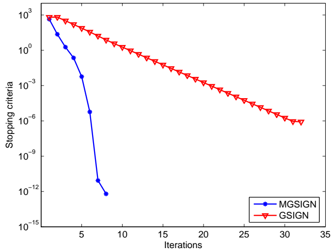
Fig. 1. Example 1: the convergence history for the generalized sign function method and the modified generalized sign function method.
