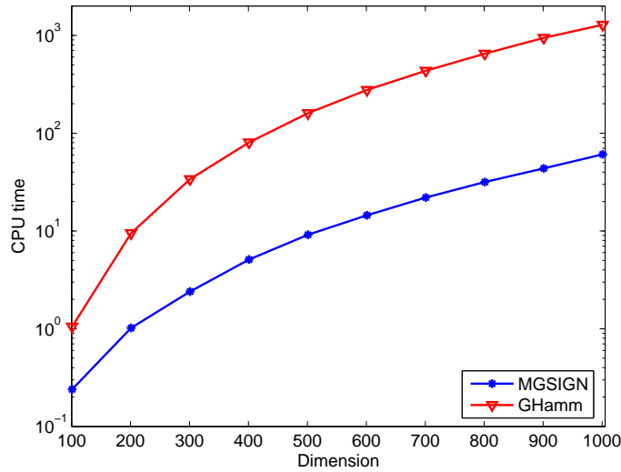
Fig. 3. Example 2: the execution time for the modified sign function method and the generalized Hammarling method.
