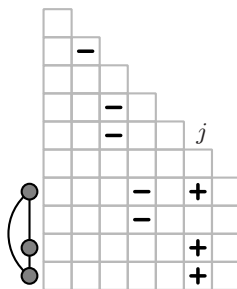
Figure 12: Combination of a clique inequality and an SCI.
