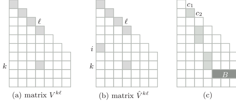
Figure 10: (a)–(b): Illustration of the matrices used in the proof of parts (1) and (3) of Proposition 14. (c): Example of an SCI that does not define a facet; see the proof of Part (4) of Proposition 14.
