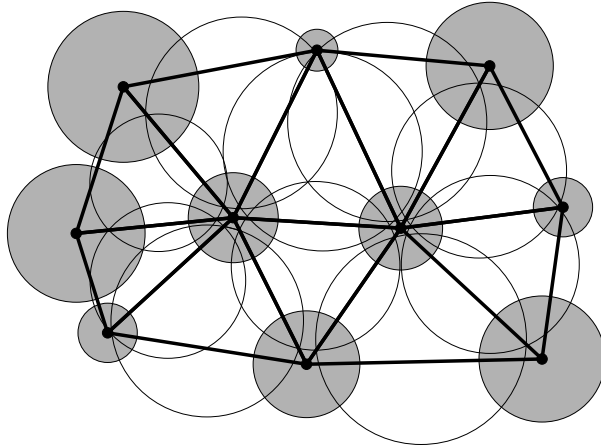
FIGURE 2. A weighted Delaunay triangulation. Note that the intersection points of two adjacent face-circles lie on the edge between them.
