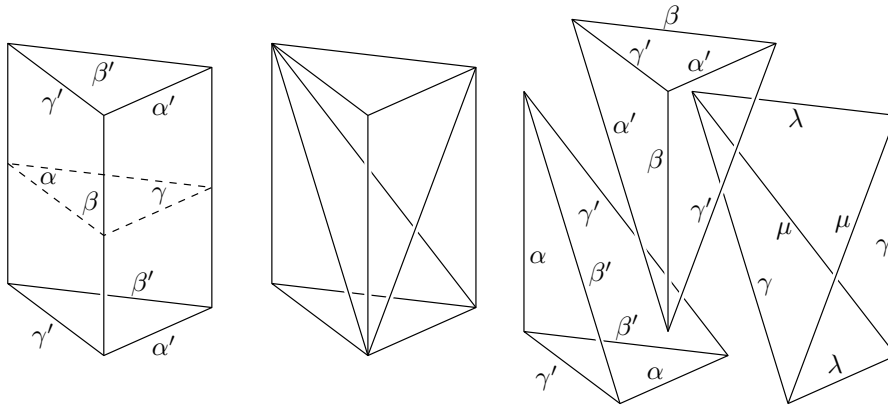
FIGURE 10. The ideal prism P_2 . To calculate its volume, we subdivide it into three ideal tetrahedra.
