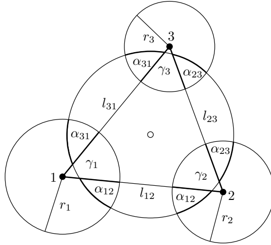
FIGURE 3. Local geometry at a triangle.
