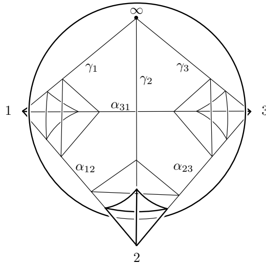
FIGURE 4. A tetrahedron in hyperbolic space (shown in the projective model) with one ideal vertex and three hyperideal vertices. The tetrahedron is truncated by the polar planes of the hyperideal vertices.
