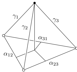
FIGURE 14. Tetrahedron with one ideal and three hyperideal vertices, partitioned into four special pyramids
