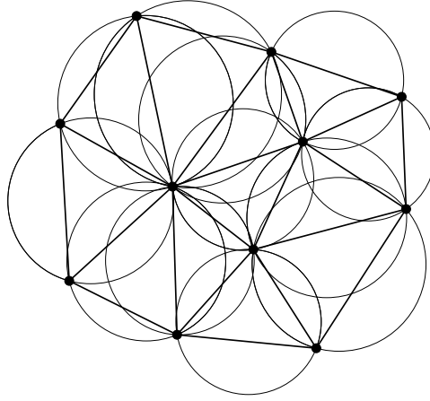
FIGURE 1. A Delaunay triangulation.
