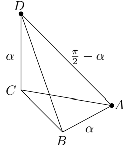
FIGURE 9. The birectangular tetrahedron P_1 with two ideal vertices A and D . The dihedral angles at the unlabeled edges are \frac{\pi}{2} .
