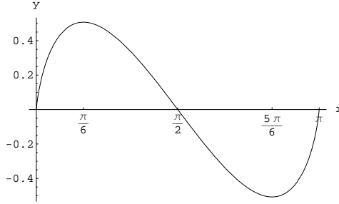
FIGURE 5. Milnor's Lobachevsky function, y = \mathbb{J}\mathbb{I}(x) .
