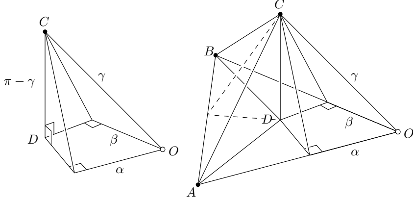
FIGURE 12. The special pyramid P_4 (left). Decomposition of a tetrahedron with one hyperideal and three ideal vertices into one special pyramid and four birectangular tetrahedra, two of which are mirror symmetric to each other (right).
