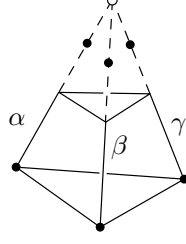
FIGURE 11. The tetrahedron P_3 with one hyperideal vertex (marked \circ ) and three ideal vertices. The points where the edges intersect the sphere at infinity are marked \bullet . The tetrahedron is truncated at the polar plane of the hyperideal vertex.
