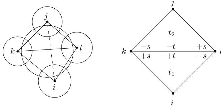
FIGURE 7. Left : If neighboring triangles share the same orthogonally intersecting circle, we can perform an edge flip. Right : How \tilde{q}(s, t) differs from \tilde{q} .
