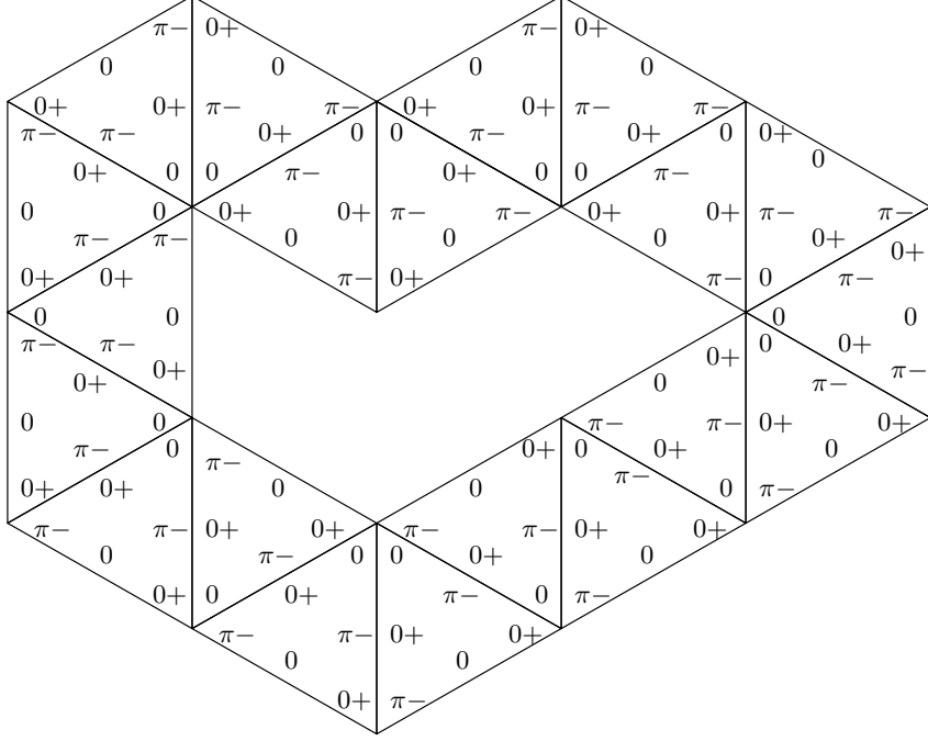
FIGURE 6. How to modify the angles along a loop of badly degenerate triangles. We write \pi- and 0+ as shorthand for “ \pi is replaced by \pi - \varepsilon ” and for “ 0 is replaced by \varepsilon ”, respectively. The changes in \alpha -angles are indicated along the edges, the changes in \gamma -angles are indicated in the corners of each triangle.
