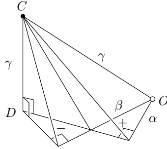
FIGURE 13. The base may also be a self-intersecting quadrilateral. Here, \beta > \frac{\pi}{2} .
