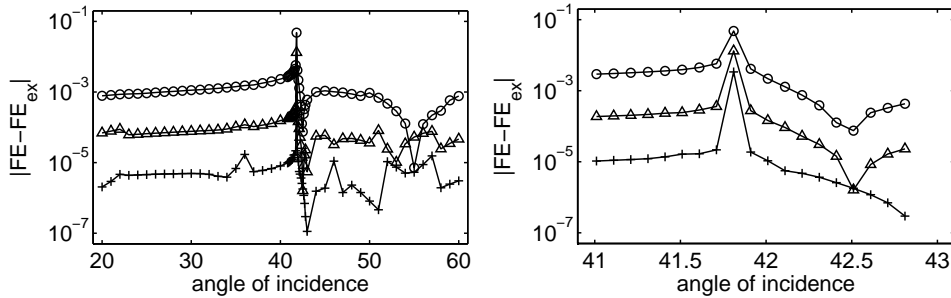
Fig. 3. Left: Field energy error in the interior domain. The three lines ( \circ , \wedge , + ) corresponds to different refinement levels of the interior domain. Right: Zoom into left figure near critical angle.
