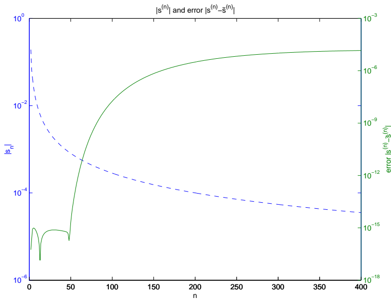
FIG. 4.1. Convolution coefficients s^{(n)} (4.12) (left axis, dashed line) and error |s^{(n)} - \tilde{s}^{(n)}| of the approximated convolution coefficients (5.1) (right axis, solid line); \rho = 1 , L = 20 .
