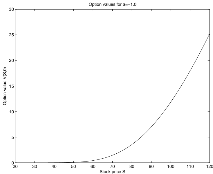
FIG. 8.1. Option values V at time t = 0 (i.e. at \tau = \tilde{T} ).
