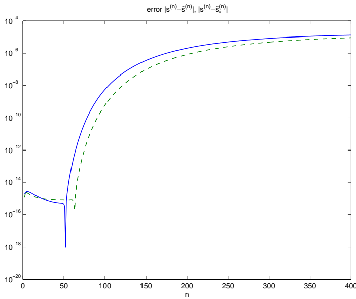
FIG. 5.1. Approximation error of the approximate convolution coefficients for \rho = 0.8 : The error of \tilde{s}_*^{(n)} (- - -) obtained from the transformation rule and the error of \tilde{s}^{(n)} (—) obtained from a direct Padé approximation of the exact coefficients s^{(n)} .
