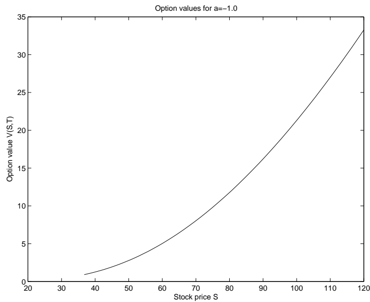
FIG. 8.5. Option values V at time t = 0 (i.e. at \tau = \tilde{T} ).
