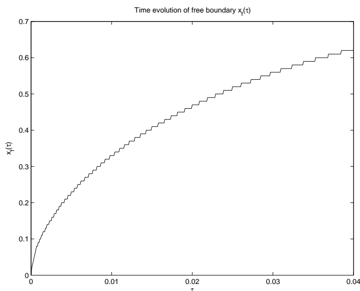
FIG. 8.2. Time evolution of the free boundary x_f(\tau) (the largest value of x_f(\tau) is about 0.62)
