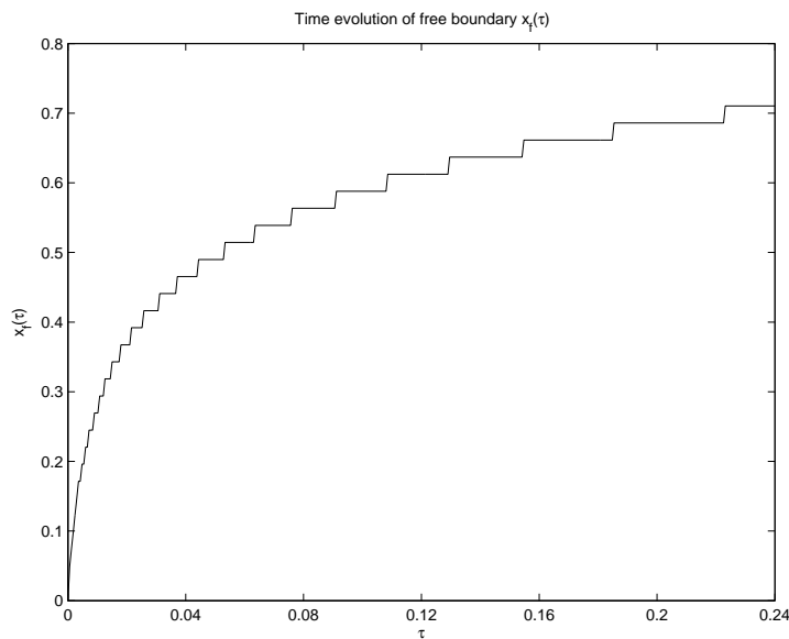
FIG. 8.6. Time evolution of the free boundary x_f(\tau) (the largest value of x_f(\tau) is about 0.71)
