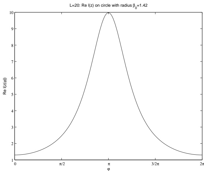
FIG. 8.3. Growth condition \operatorname{Re} \hat{\ell}(z = \beta e^{i\varphi}) \geq 1 for the approximated discrete transparent boundary condition of §5 with L = 20 . The stability condition (7.3) is satisfied for all \beta \geq 1.42
