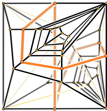
FIGURE 17: The outcome of step 2 of the construction: The cubical convex 3-ball \mathcal{B}_{14} which contains a Möbius strip with parallel inner edges in the 2-skeleton.
