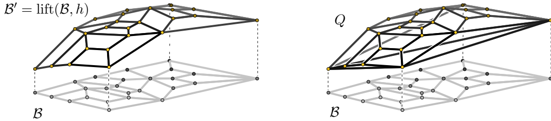
FIGURE 10: A lifted cubical ball (\mathcal{B}, h) and its lifted copy \text{lift}(\mathcal{B}, h) . The figure on the right shows the convex hull Q = \text{conv}(\text{lift}(\mathcal{B}, h)) .
