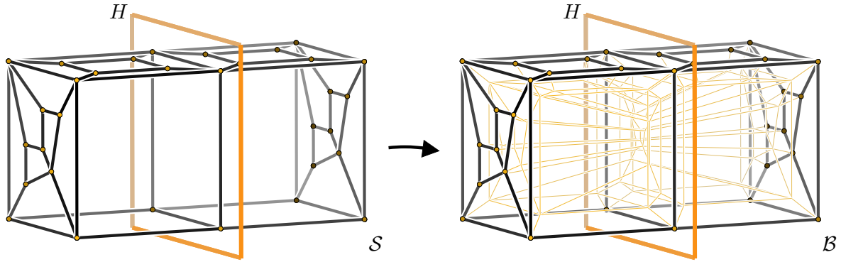
FIGURE 18: The Hexhoop template of Yamakawa & Shimada [32].
