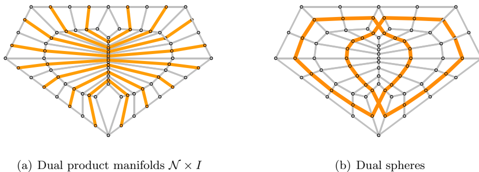
FIGURE 28: The dual manifolds of a 2-dimensional generalized regular Hexhoop.
