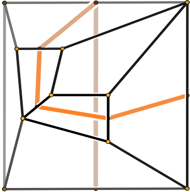
FIGURE 15: The cubical octahedron O_8 positioned in \mathbb{R}^3 with a regular square base facet Q and acute dihedral angles at this square base. A part of one dual manifold is highlighted.
