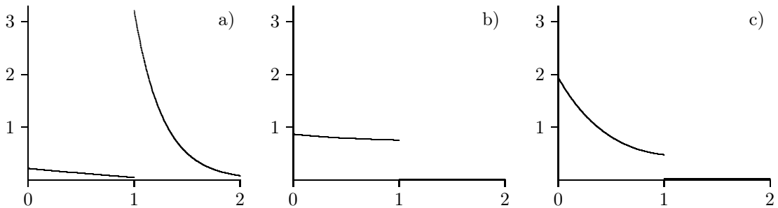
Figure 2: Graphs on [0, 2] of the density f_L of the residence time distribution in normalized time. Parameters of the original model: r = 500 , a) \sigma = 0.30 , \beta = 0.1 , b) \sigma = 0.30 , \beta = -0.1 , c) \sigma = 0.35 , \beta = -0.1 .
