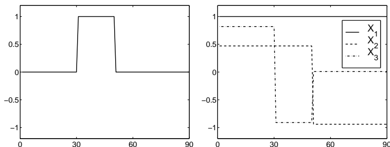
Figure 1: Uncoupled Markov chain over k = 3 disjoint index subsets. The state space \mathcal{S} = \{s_1, \dots, s_{90}\} divides into the index subsets \mathcal{S}_1 = \{s_1, \dots, s_{29}\} , \mathcal{S}_2 = \{s_{30}, \dots, s_{49}\} , and \mathcal{S}_3 = \{s_{50}, \dots, s_{90}\} . Left: Characteristic function \chi_2 . Right: Eigenbasis \{X_1, X_2, X_3\} corresponding to 3-fold eigenvalue \lambda = 1 .
