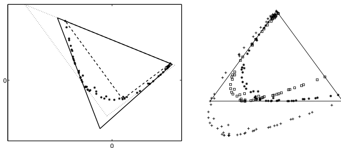
Figure 5: Artificial example. Left: input data (*) in simplex \tilde{\sigma}_2 . Initial simplex guess (- - -), rescaled initial guess (⋯), and final iterate (—). Right: almost characteristic function values in simplex \sigma_2 . Initial guess (+), rescaled initial guess (□), and final iterate (*).
