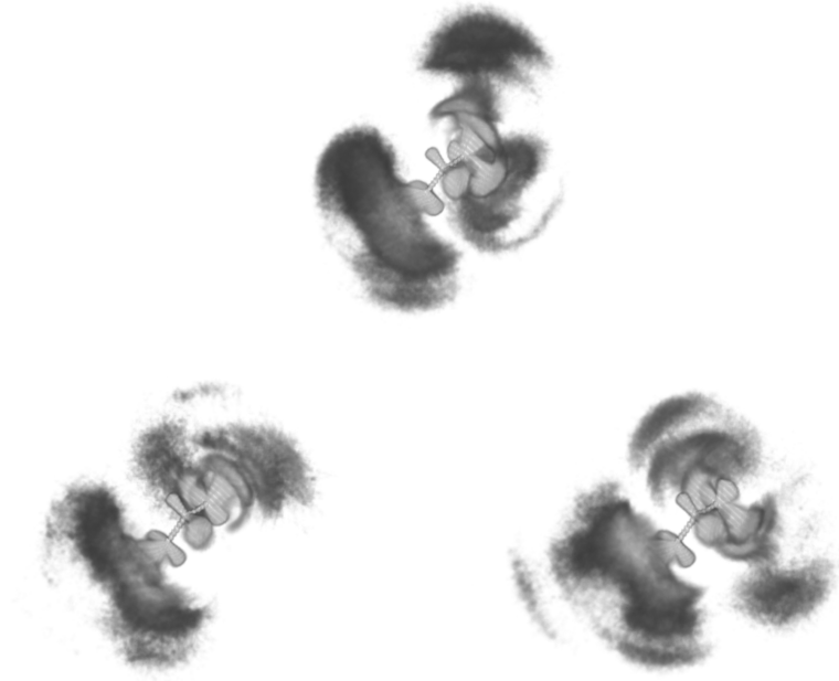
Figure 6: HIV protease inhibitor . Top : conformation 1. Bottom left : conformation 2. Bottom right : conformation 3.
