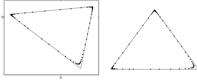
Figure 7: HIV protease inhibitor: eigenvectors and almost characteristic function values. Left: input data and final iterate simplex \tilde{\sigma}_2 . Observe the occurrence of 'dirty zero' data. Right: almost characteristic function values in simplex \sigma_2 .
