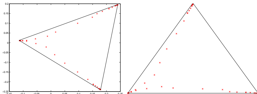
Figure 3: Butane molecule ( k = 3 ): Left : Simplex \tilde{\sigma}_2 containing (\tilde{X}_2(l), \tilde{X}_3(l)) , l = 1, \dots, N . Observe the occurrence of 'dirty zero' data in the left corner. Right : Simplex \sigma_2 for almost characteristic functions (\tilde{\chi}_1, \tilde{\chi}_2, \tilde{\chi}_3) .
