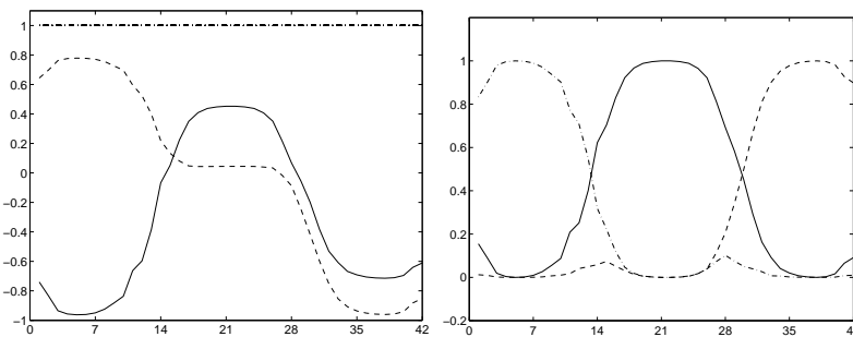
Figure 4: Butane molecule ( k = 3 ): Left : Perron cluster eigenvectors \tilde{\chi}_1 = e, \tilde{\chi}_2, \tilde{\chi}_3 to Perron cluster eigenvalues \tilde{\lambda} = 1, 0.99, 0.98 . Observe the occurrence of 'dirty zero' data in the range \{16, \dots, 26\} . Right : Perturbed characteristic functions \tilde{\chi}_1, \tilde{\chi}_2, \tilde{\chi}_3 .
