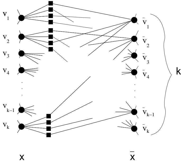
Fig. 2. edge gadgets of variable x after identification of the terminals
