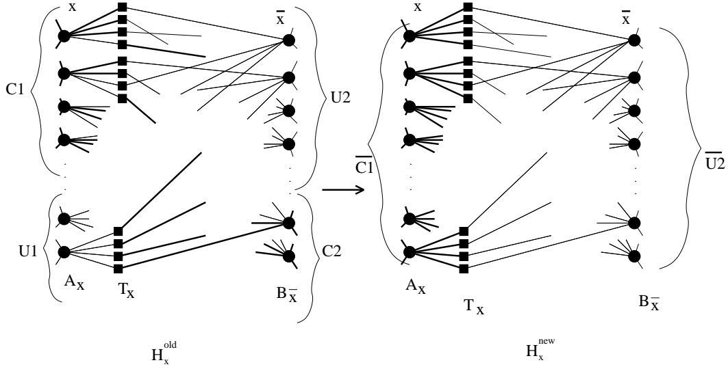
Fig. 5. Modification of the edges of the Steiner tree in the edge gadgets
