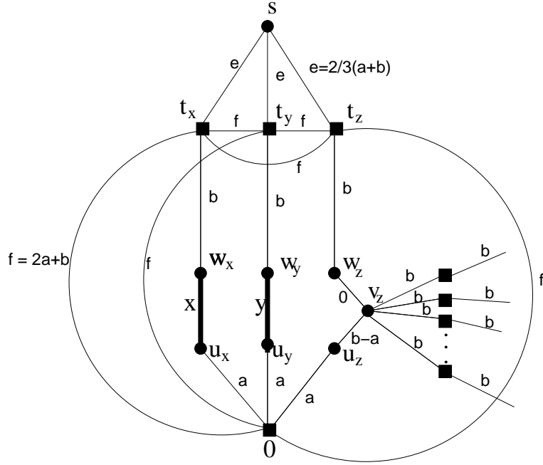
Fig. 3. edge weights (edge gadget for z inserted)
