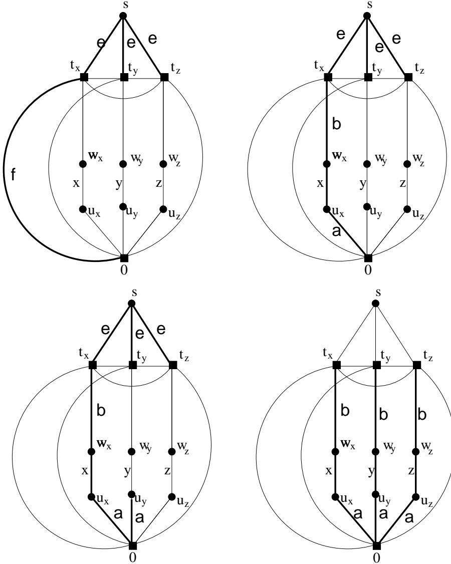
Fig. 4. The four cases of optimal subtrees
