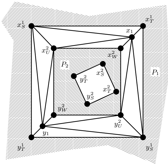
Figure 4: Gluing two almost-triangulations P_1 and P_2
