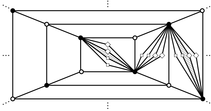
Figure 1: A quadrangulation P_S which corresponds to a star S with three leaves. The black vertices belong to U_1 . The shaded faces indicate a possible choice for \mathcal{C}_1 .
