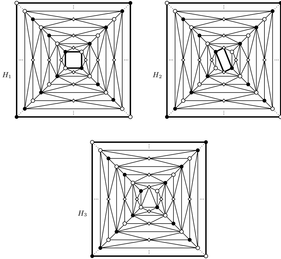
Figure 3: The graphs H_1 , H_2 and H_3 , the only non-triangular facial cycles are indicated with thick lines
