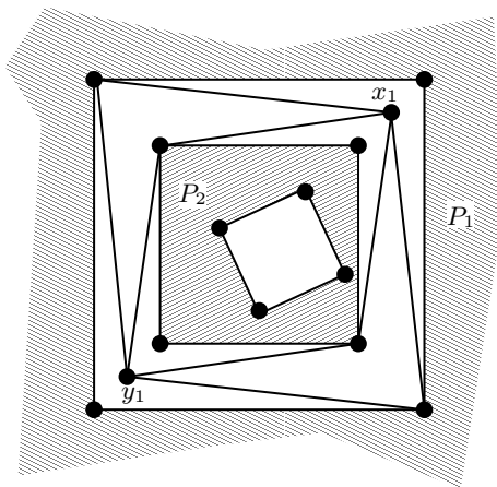
Figure 5: Gluing two quadrangulations P_1 and P_2
