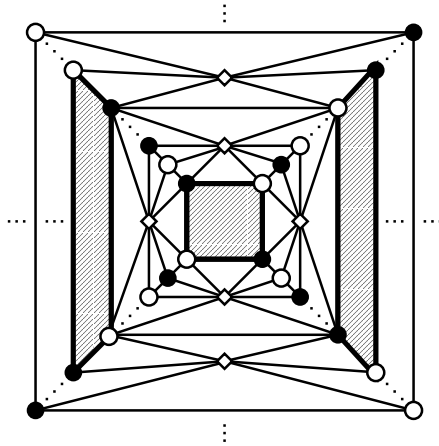
Figure 2: A triangulation apart from the shaded faces (into which the exceptional vertices will be inserted)
