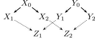
Figure 6: An unsatisfiable dominance graph.
