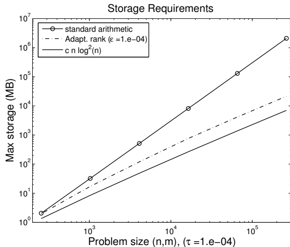
Figure 1: Maximal storage requirements in logarithmic scale for Algorithm 1 in \mathcal{H} -matrix arithmetic and in standard arithmetic compared to an \mathcal{O}(n \log^2 n) reference line.
