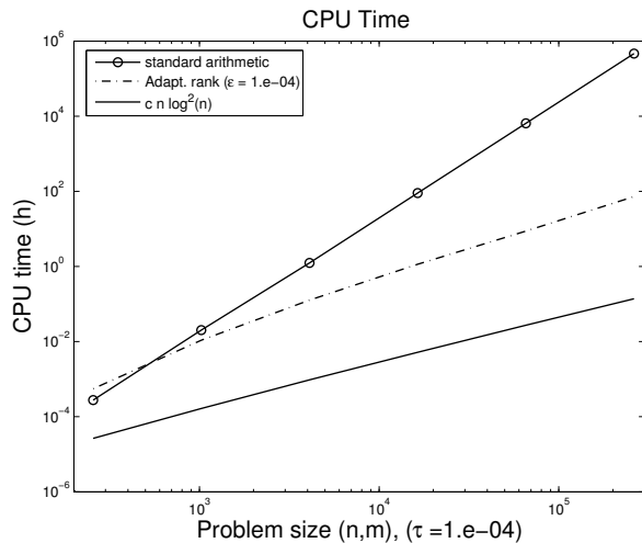
Figure 2: CPU time in logarithmic scale for Algorithm 1 in \mathcal{H} -matrix arithmetic and in standard arithmetic compared to an \mathcal{O}(n \log^2 n) reference line.
