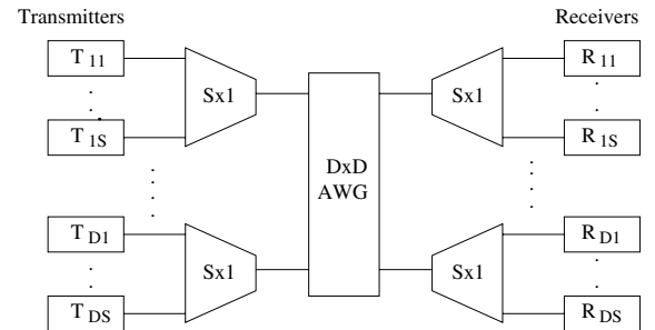
Fig. 1. Network architecture
